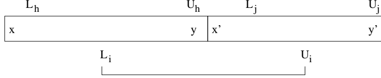
Fig. 11. An example of a typical search range, [L_i, U_i] , that lies across two adjacent blocks, [x, y] and [x', y'] .
